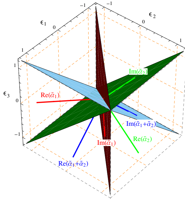
Figure 1. Real and imaginary parts of the A_2 deformed roots divided by R(\varepsilon) and I(\varepsilon) , respectively, in the three-dimensional standard representation for the simple roots \alpha_1 = \varepsilon_1 - \varepsilon_2 , \alpha_2 = \varepsilon_2 - \varepsilon_3 . Both parts of a particular positive root \tilde{\alpha}_i are depicted in the same color (on-line).
